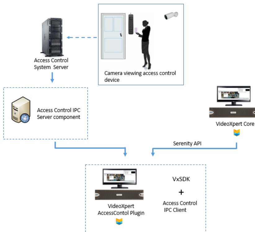
Figure 1: Access Control System overview
