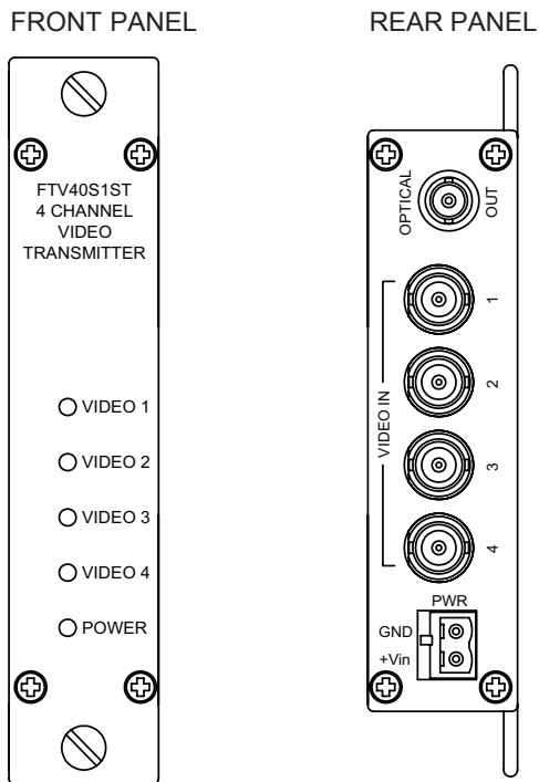
FIGURE 2 – TRANSMITTER
