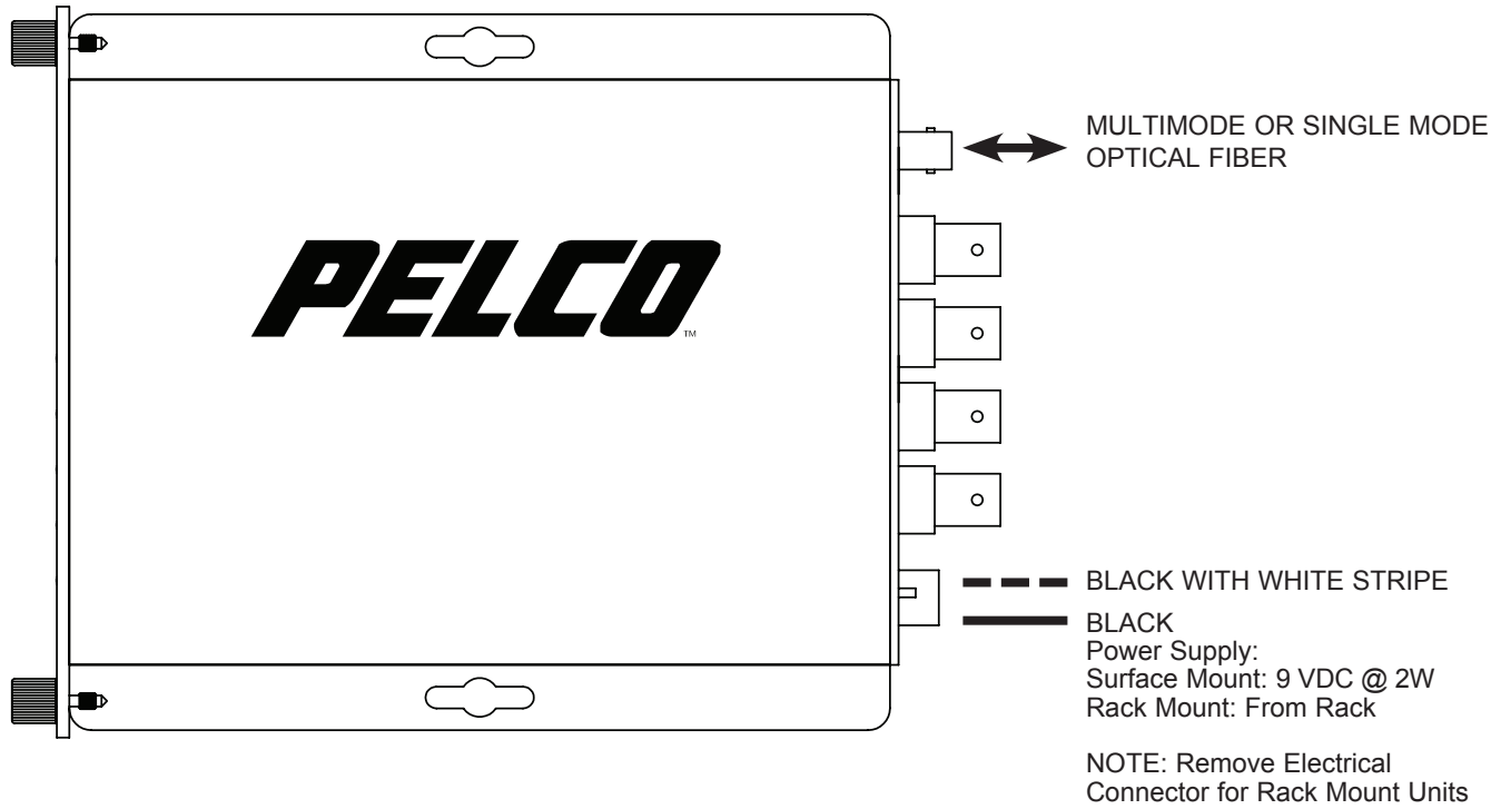
FIGURE 1 – FTV/FRV40(M,S)1(ST,FC) TRANSMITTER AND RECEIVER
