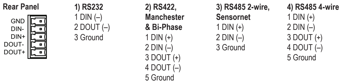
FIGURE 6 – DATA CONNECTIONS
