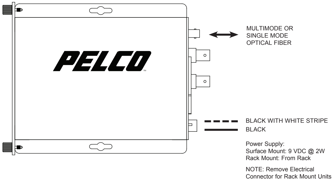
FIGURE 1 – FTV/FRV10D1A2(M,S)1(ST,FC) TRANSCEIVER
