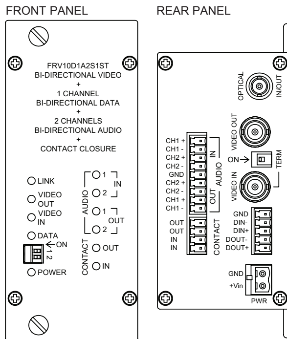
FIGURE 2 – RECEIVER
