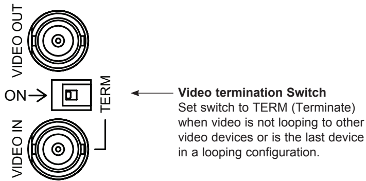
FIGURE 3 – VIDEO TERMINATION SWITCH
