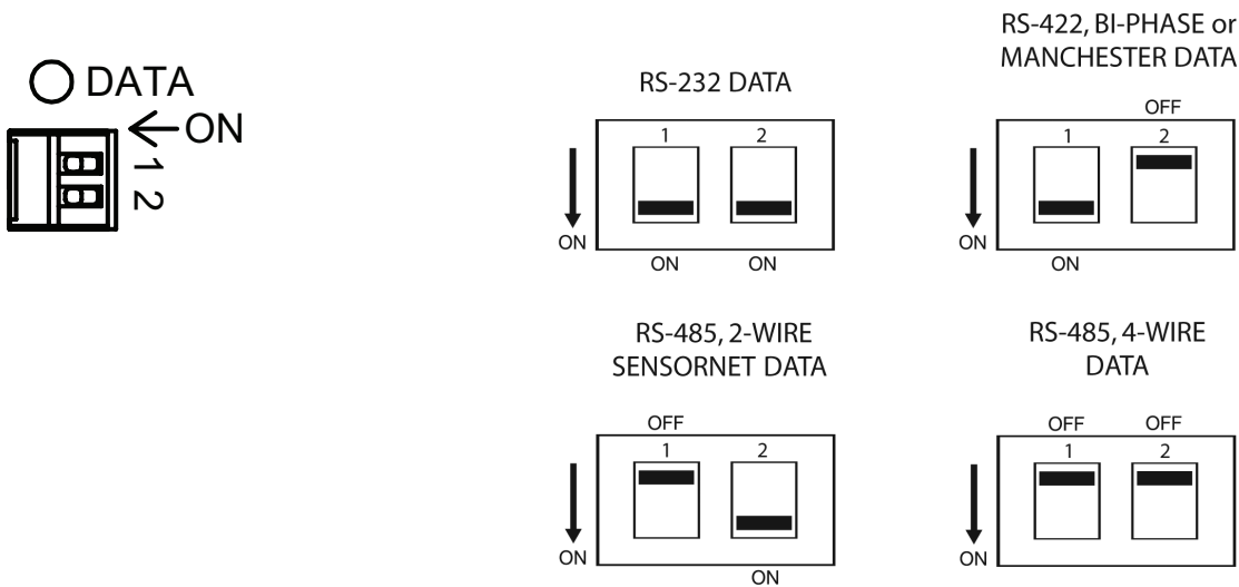
FIGURE 4 – SWITCH POSITIONS
