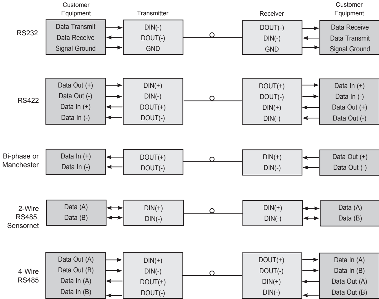
FIGURE 5 – DATA CONNECTIONS
