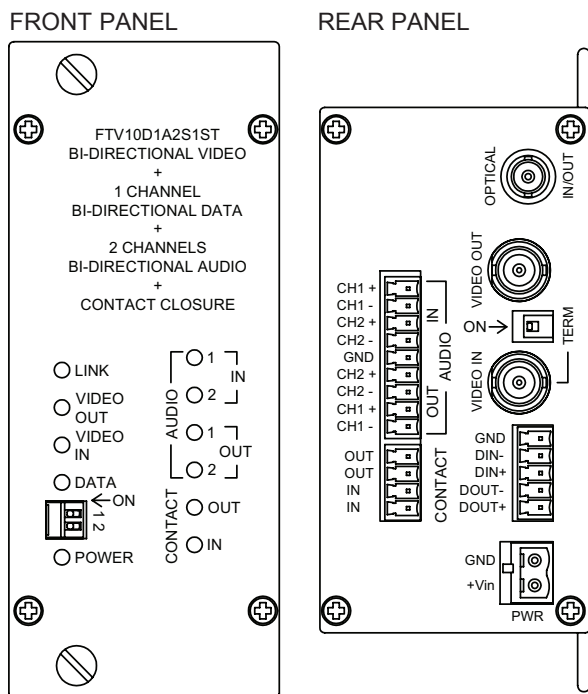
FIGURE 2 – TRANSMITTER
