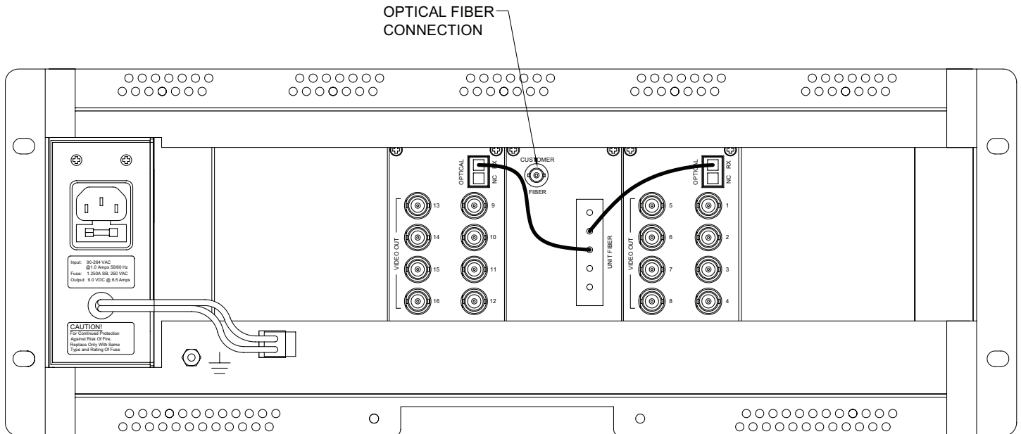
FIGURE 2 – FRV160(M,S)1(ST,FC) FRONT AND REAR
