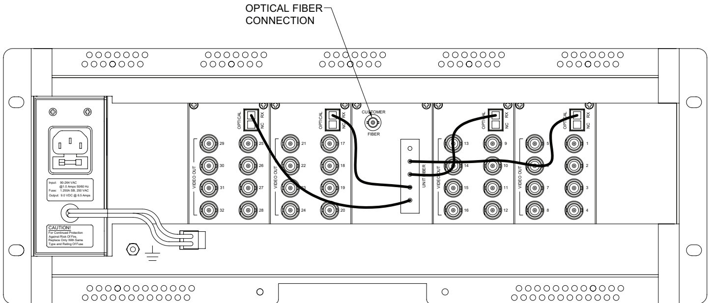
FIGURE 4 – FRV320(M,S)1(ST,FC) FRONT AND REAR
