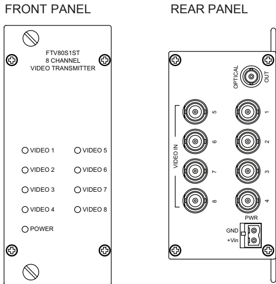
FIGURE 2 – TRANSMITTER
