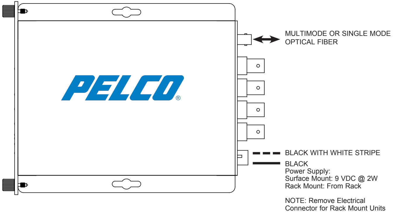
FIGURE 1 – FTV/FRV80(M,S)1(ST,FC) TRANSMITTER AND RECEIVER
