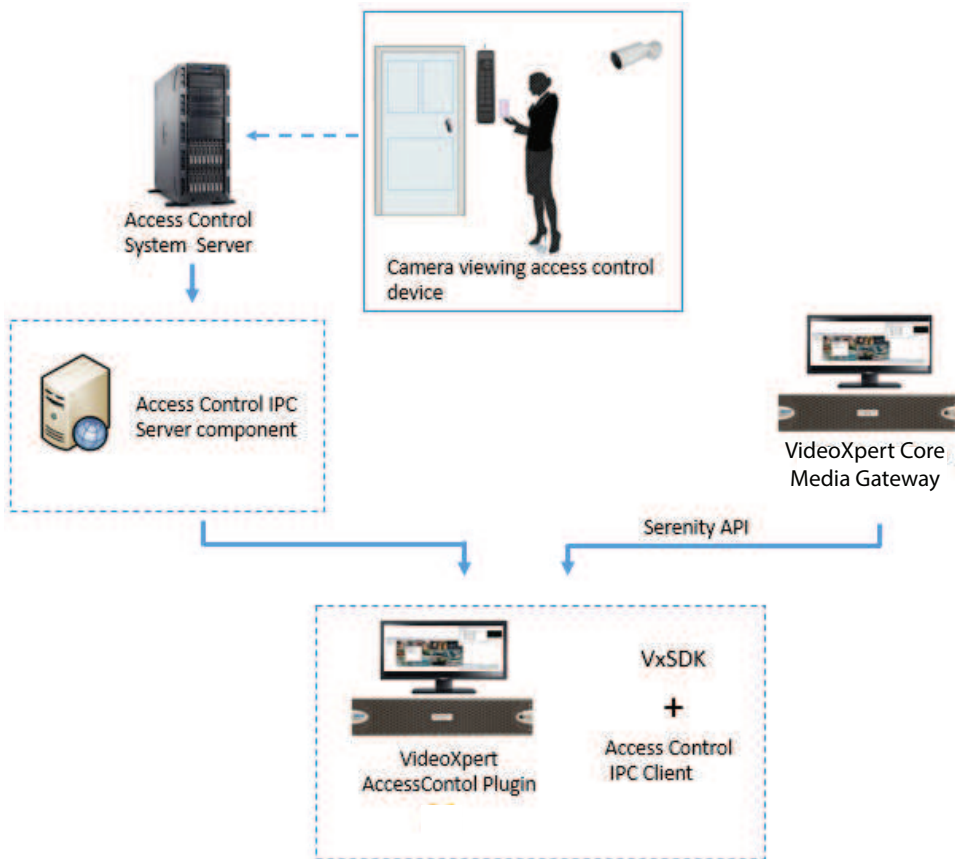
Figure 1: Access Control System overview
