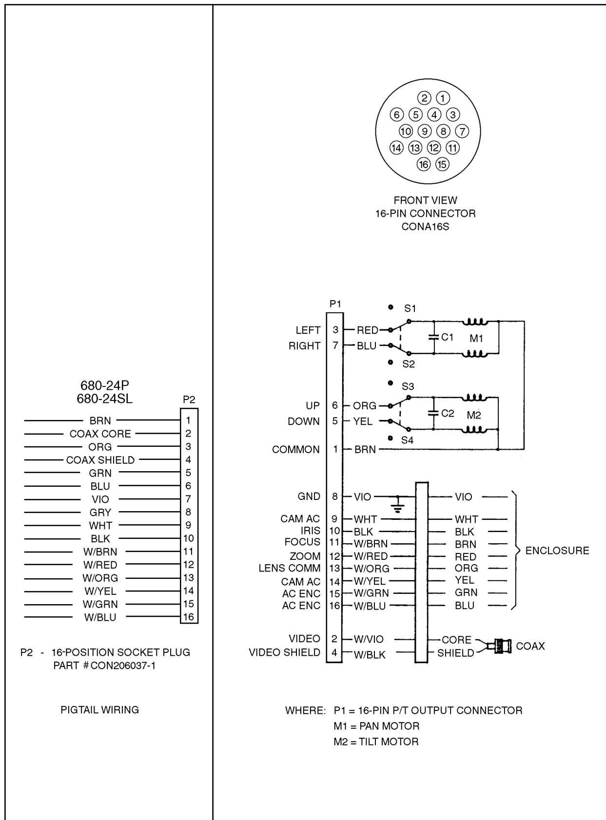
Figure 12. PT680-24P Wiring Schematic
