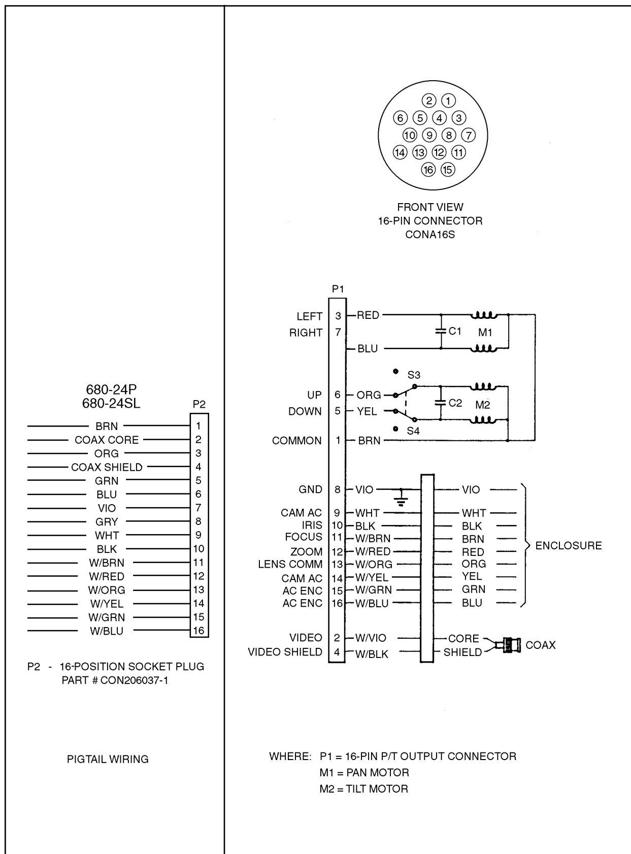
Figure 13. PT680-24SL Wiring Schematic
