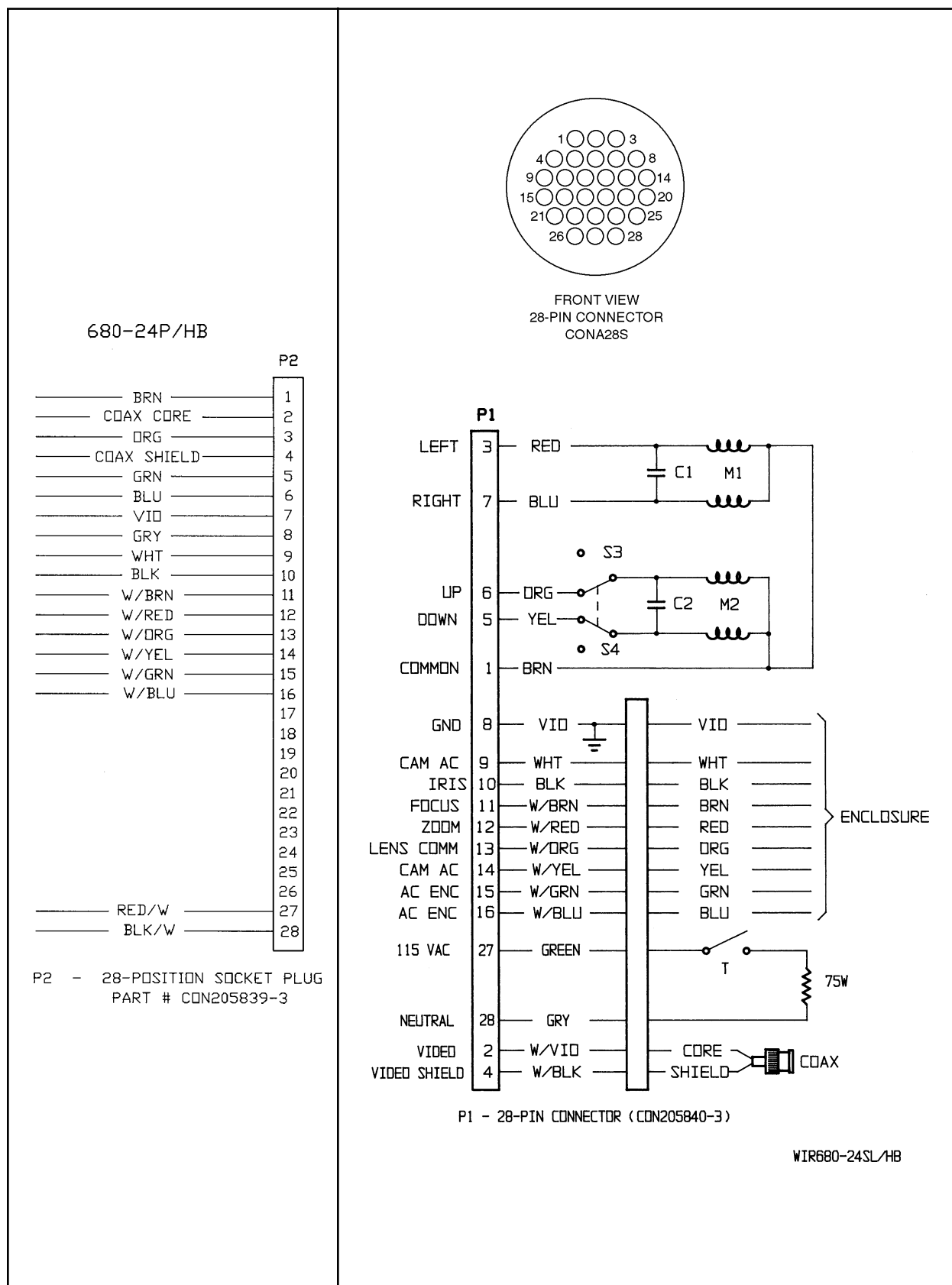
Figure 17. PT680-24SL/HB Wiring Schematic
