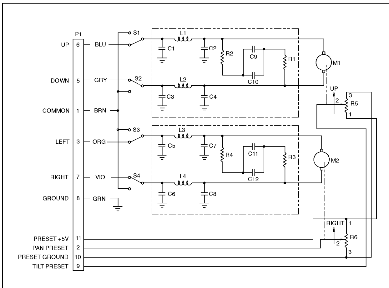
Figure 9. PT550P/PP Wiring Diagram
